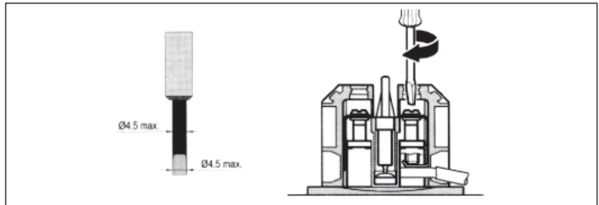
Figure 3: Fixing the supply cable.
