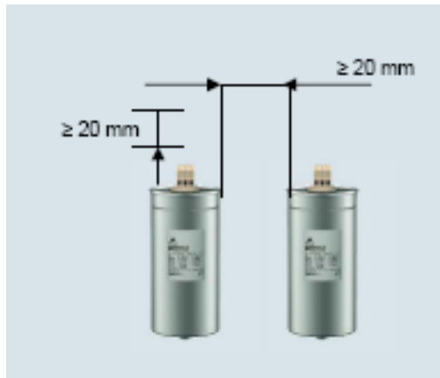
Figure 2: Minimum space over and between the capacitors.
